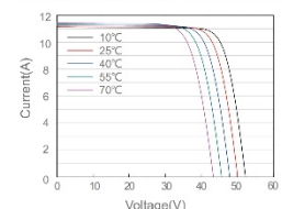
Current-Voltage Curve JAM72D20-440/MB
